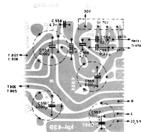
Elkoplatte, Bestückungsseite ELECTROLYTIC CAPACITOR BOARD, COMPONENT SIDE PLAQUE CONDENSATEURS ELECTROLYTIQUES, VUE DU COTE DES COMPOSANTS PIASTRA COND. ELETTROLITICI, LATO COMPONENTI
